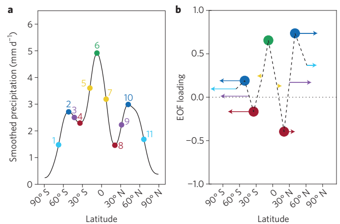
Figure 3 | Simulated process-based fingerprint of anthropogenic precipitation change. a , Zonal mean boreal winter precipitation observations for 1990. Local extrema are marked in dark blue (mid-latitude storm tracks), red (subtropical dry zones), and green (equatorial tropical peak). Cyan, purple, and yellow circles indicate half-max points. b , Multivariate fingerprint of forced precipitation change as thermodynamic and dynamic process indicators. The thermodynamic empirical orthogonal function (EOF) loading is plotted on the vertical axis and the direction and magnitude of dynamic EOF loading are displayed as arrows showing the wet-gets-wetter and dry-gets-drier pattern in precipitation intensity and the poleward extension of precipitation over storm track and subtropical arid latitudes in both hemispheres 48 . Figure reproduced with permission from ref. 47, © 2013 PNAS.
