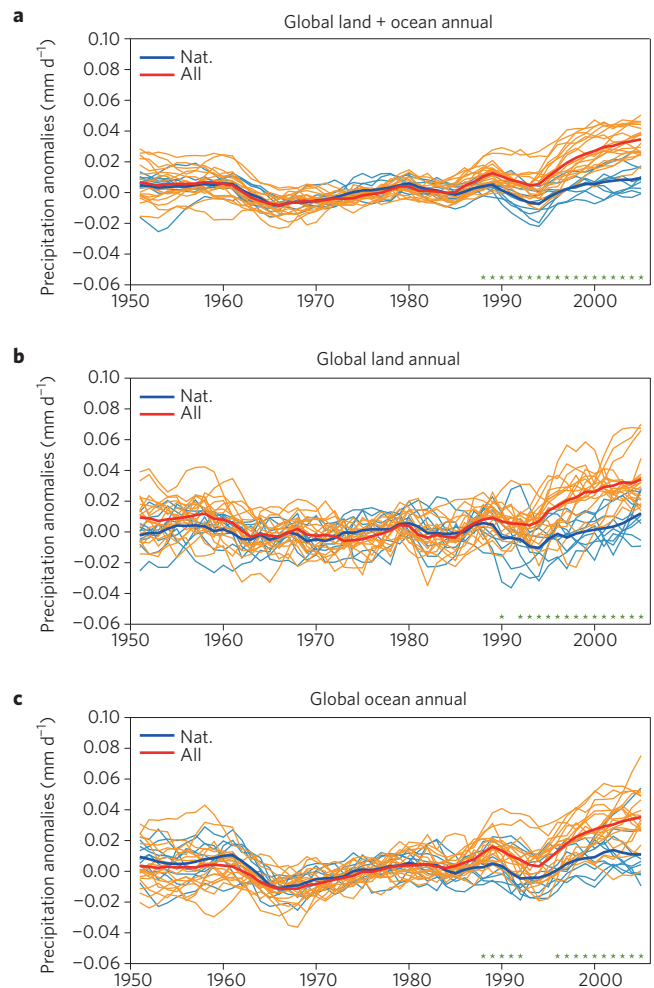
Figure 1 | Observational uncertainties due to sparse coverage obscure expected fingerprints of change. a–c, Time-series of global mean precipitation anomalies ( \text{mm d}^{-1} ) with respect to the baseline period of 1961–1990, simulated by CMIP5 models forced with both anthropogenic and natural forcings (All; orange/red lines) and natural forcings only (Nat., blue lines).
