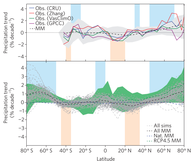
Figure 2 | Magnitudes of zonal mean land precipitation trends are dependent on observational datasets. Comparison of observed trends (Obs., solid lines) using 4 observational datasets 11,80–82 for 1951–2005 (top). The ranges of CMIP5 simulations are in grey shading and the multi-model ensemble mean (MM) is a black dashed line. The blue (orange) shadings show latitudes where all observed datasets show positive (negative) trends. Comparison of simulated trends (sims; bottom) using CMIP5 historical (All) simulations (individual simulations shown by grey dashed lines; multi-model mean shown by the black dashed line), and the natural forcing only (Nat.) simulations (MM; blue dashed line) with the future (2006–2050) trend using RCP4.5 simulations (5–95% range is in green shading; MM in green dashed lines). Blue (orange) shading indicates latitudinal regions where more than two-thirds of the historical simulations show positive (negative) trends 4 . Figure reproduced with permission from ref. 4, © 2015 AMS.
